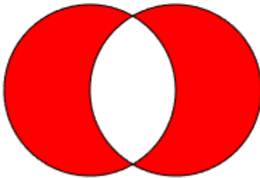
Exclusive Or
