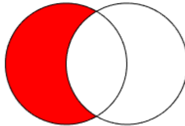
Subtraction
