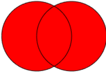
Union
