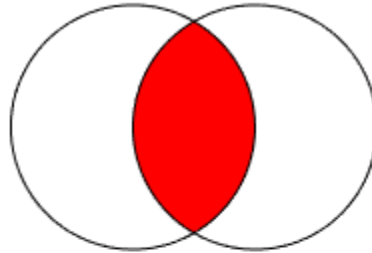
Intersection
